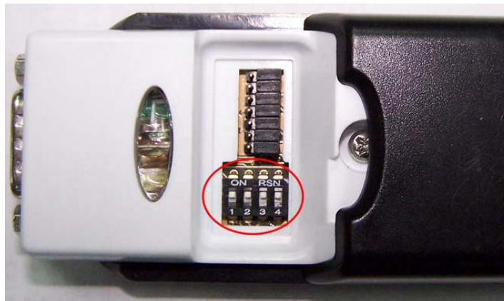
4-pin DIP switch for operating mode selection
