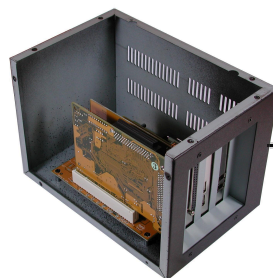
Installing PCI Add-in cards inside the Expansion Box
